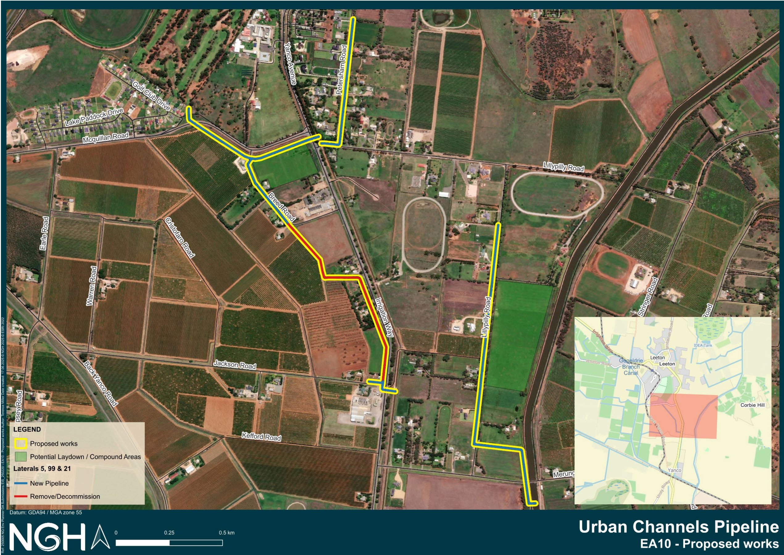
Figure 2-2 Proposed works
