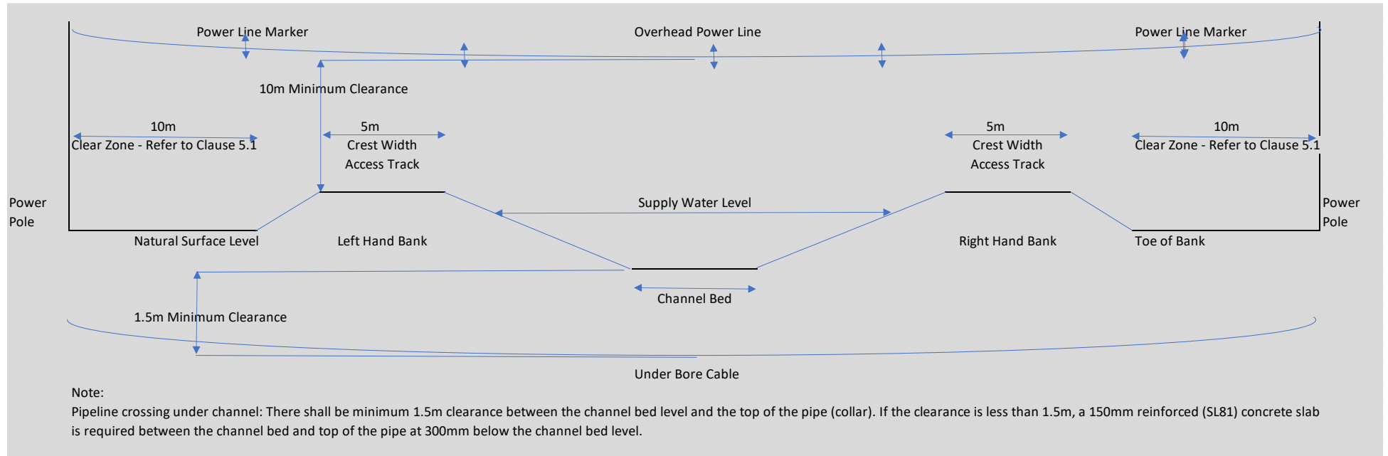
Diagram 1- This illustration is provided as a guide for Crest Width and Toe of the Bank
